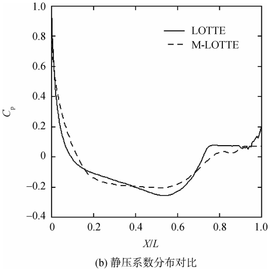
图 9 LOTTE 和 M-LOTTE 飞艇中心截面气动性能分布对比 Fig. 9 Comparison of aerodynamic performance on the central cross-section of LOTTE and M-LOTTE airships
