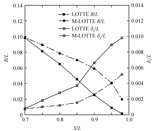
图 10 LOTTE 和 M-LOTTE 飞艇艇身半径和动量边界层厚度 Fig. 10 Body radius and momentum boundary thickness for LOTTE and M-LOTTE airships
