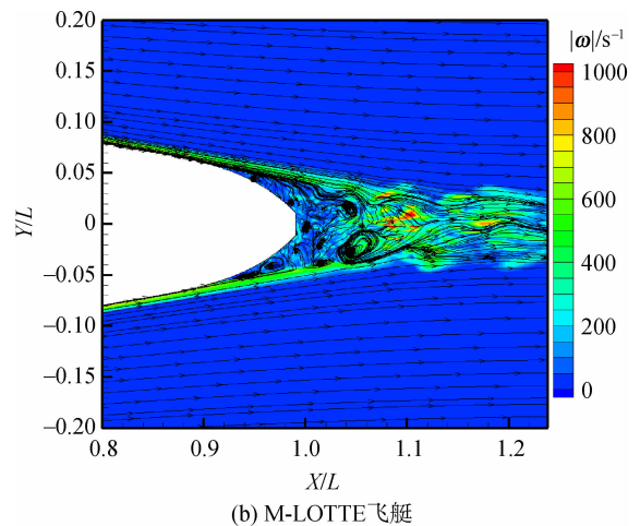
图 4 LOTTE 和 M-LOTTE 飞艇中心截面流线和涡量分布 Fig. 4 Streamlines and vorticity distribution for LOTTE and M-LOTTE airships at central cross-sections
