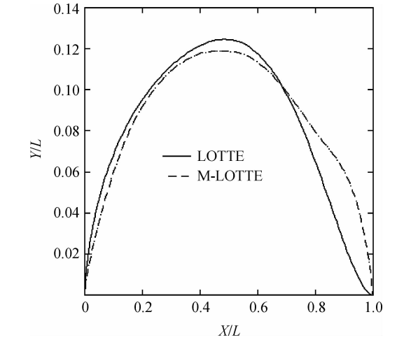
图 3 LOTTE 和 M-LOTTE 形状对比 Fig. 3 Comparison of LOTTE and M-LOTTE airships hull
