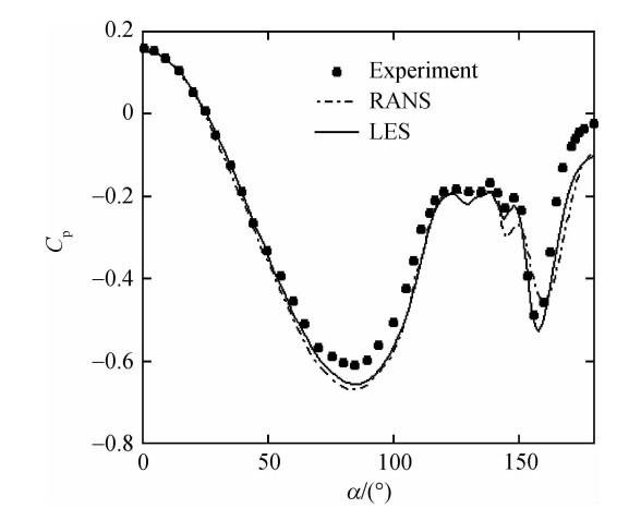
图 2 椭球体在 X/L=0.56 截面处静压系数分布的比较 Fig. 2 Comparison of static pressure coefficient distribution for cross-section of spheroid at X/L=0.56
