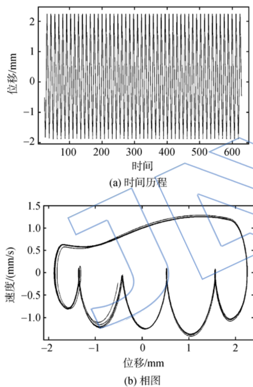
图 4 冠间间隙失谐下的叶片共振响应 Fig. 4 Resonant response of blades with mistuning tip clearance
