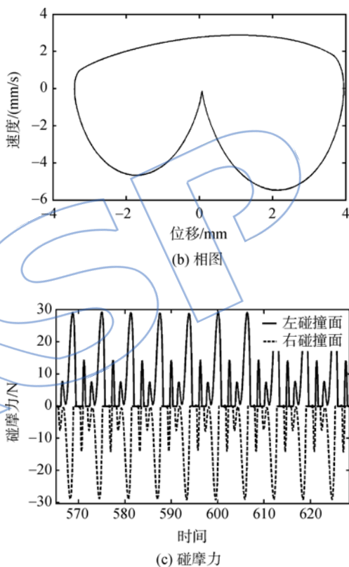
图 6 第 13 阶共振频率下振动响应特性和碰摩力 Fig. 6 Vibration response characteristics and rub-impact force at the 13th order resonant frequency
