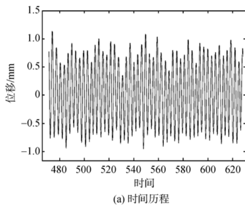
图 6 第 13 阶共振频率下振动响应特性和碰摩力 Fig. 6 Vibration response characteristics and rub-impact force at the 13th order resonant frequency
