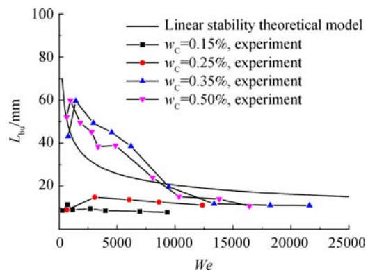
图 11 4 种卡波姆凝胶在不同 We 下的破碎长度曲线 Fig. 11 Breakup length curves of four kinds of Carbopol gel with different Weber numbers
