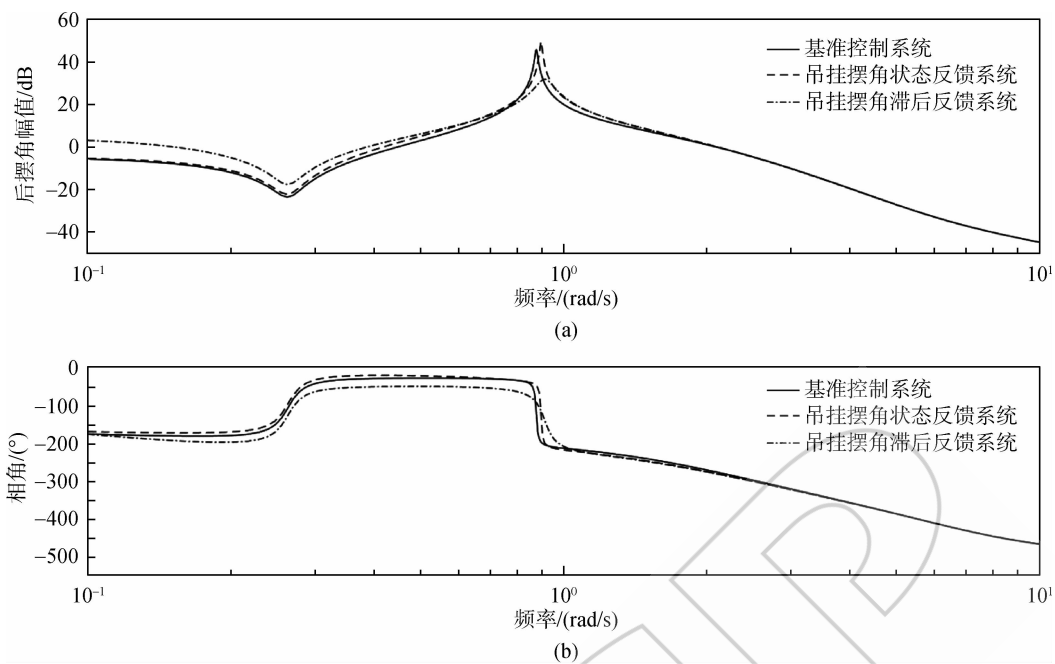
图 5 吊挂后摆角在横向操纵输入下的波特图 Fig. 5 Bode diagram of rear swing angle due to lateral cyclic
