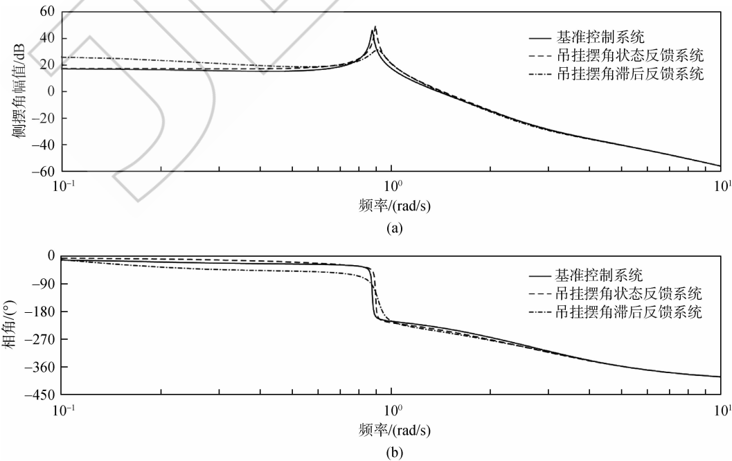
图 4 吊挂侧摆角在横向操纵输入下的波特图 Fig. 4 Bode diagram of lateral swing angle due to lateral cyclic
