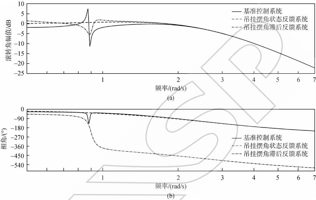
图 3 滚转角在横向操纵输入下的波特图 Fig. 3 Bode diagram of roll attitude angle due to lateral cyclic
