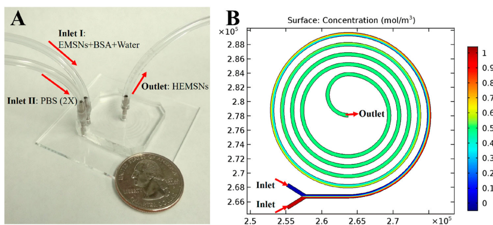
Figure 2. (A) Experimental set-up for the microfluidic synthesis of HEMSNs, with a quarter-dollar coin for scale. (B) Comsol simulation result of mixing in the microfluidic spiral channel, where two flows having different concentrations could achieve complete mixing within about one run (see simulation details in SI).
