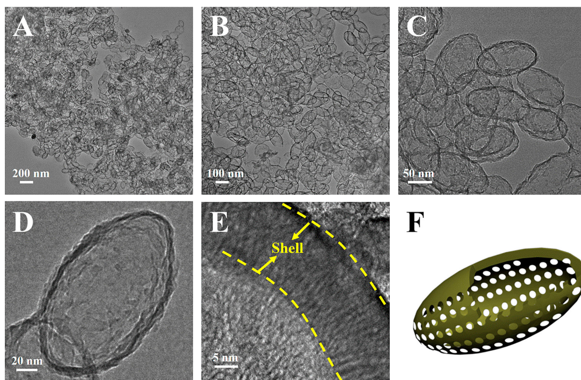
Figure 3. (A–E) TEM images of HEMSs at different magnifications. (F) A schematic illustration of the hollow ellipsoidal nanoparticle with typical shell and inner void.
