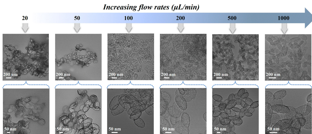
Figure 4. The effect of the flow rates (i.e. etching time) on the morphological changes of EMSNs.
