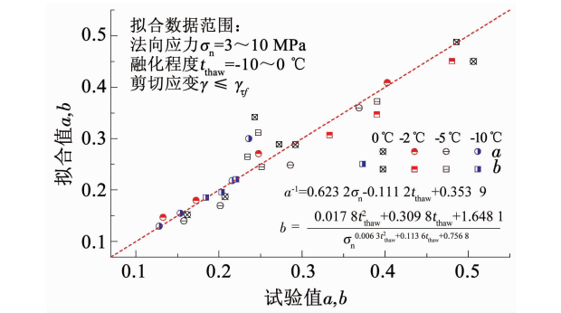
图 11 双曲线模型拟合 a, b 和实测值比较 Fig. 11 Comparison of fitting results of hyperbolic model with measured values
