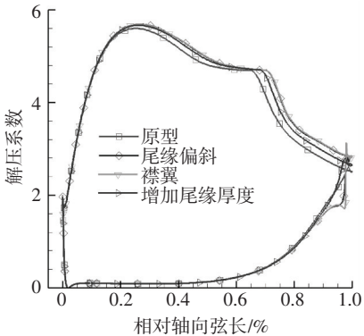
图 7 Re=20\,000 时静压系数分布 Fig.7 Static pressure coefficient distribution, Re = 20\,000
