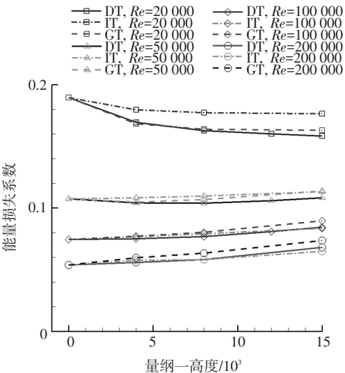
图 5 量纲一高度对叶栅能量损失系数的影响 Fig.5 Effects of dimensionless height on the energy loss coefficient
