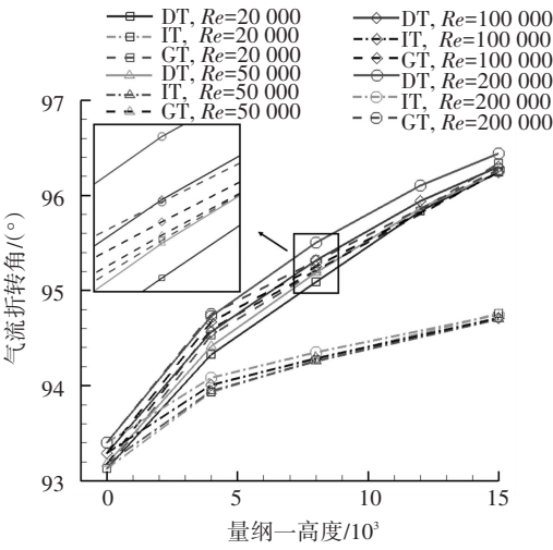
图 6 量纲一高度对叶栅气流折转角的影响 Fig.6 Effects of dimensionless height on the flow turning angle
