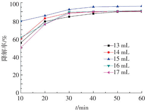
图 8 加入不同过氧化氢时亚甲基蓝降解率 Fig.8 Degradation rate of MB with reacted time with different initial amount of H 2 O 2
