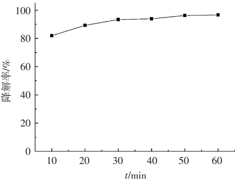
图 11 最优条件下亚甲基蓝降解率与时间关系 Fig.11 Variation of photo-Fenton degradation rate of MB with reacted time
