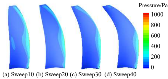
图 12 起飞状态后桨吸力面静压的 2 阶谐波 Fig. 12 The 2nd harmonic pressure distributions of rear blade suction-surface at take-off condition
