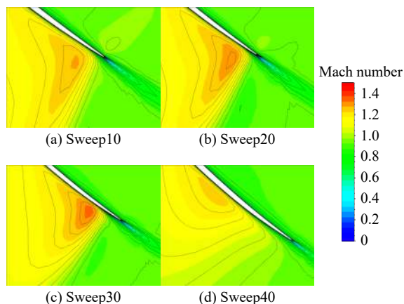
图 5 巡航状态下前桨 95% 叶高马赫数分布 Fig. 5 Mach number distributions of front blade at 95% span at cruise condition
