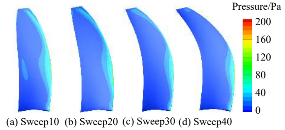
图 13 起飞状态后桨吸力面静压的 3 阶谐波 Fig. 13 The 3rd harmonic pressure distributions of rear blade suction-surface at take-off condition
